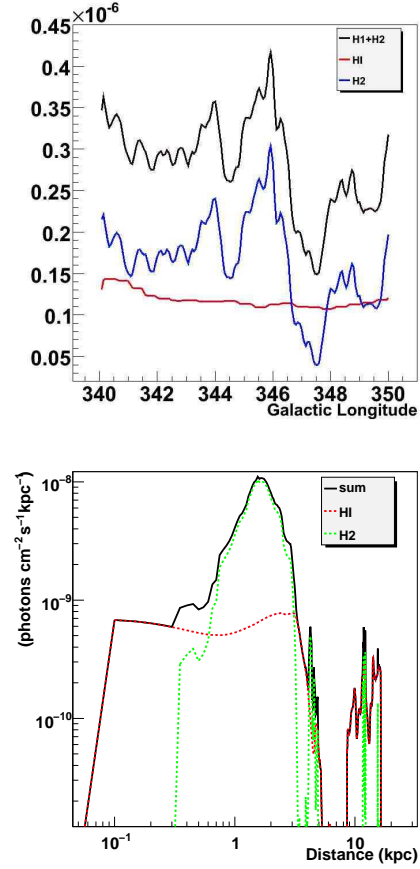
Fig. 1. ( Top ) The longitudinal profile of the \gamma -ray emission from the region 340^\circ < l < 350^\circ , integrated over the latitude range -5^\circ < b < 5^\circ . The dotted green lines are for the emission arising from CRs scattering off molecular hydrogen, the dashed red ones for the emission arising from CRs scattering off atomic hydrogen and the solid black ones for the sum. ( Bottom ) Flux above 1 GeV as function of the line of sight distance, produced by CRs interacting with the atomic and molecular gas. (Casanova et al 2010a)
