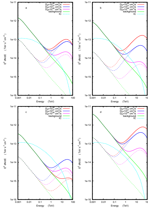
Fig. 2. The \gamma -ray energy flux in four different regions of 0.2 \times 0.2 degrees around the positions a = (346.8, -0.4), b = (346.9, -1.4), c = (347.1, -3.0) and d = (346.2, 0.2). The emission produced along the line of sight distance between 900 and 1100 parsecs is plotted in dashed lines, while the emission obtained by summing the radiation contributions over the whole line of sight distance, from 50 parsecs to 30000 parsecs, is shown in solid lines. The emission in the panels a,b,c and d, corresponding to the different locations, is plotted for different diffusion coefficients D_0 . The emission from background CRs is also shown in each panel for comparison. The contribution to the emission from inverse Compton scattering of background electrons is indicated with a dashed light blue line.
