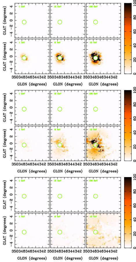
Fig. 3. Ratio of the emission due to the sum of background CRs and runaway CRs and background CRs only. The SNR is supposed to have exploded at 1 kpc distance from the Sun at 347.3^\circ longitude and -0.5^\circ latitude 1600 years ago and to have started injecting the most energetic protons 100 years after the explosion (Zirakashvili, V.N. & Aharonian 2010). The diffusion coefficient assumed within the region 340^\circ < l < 350^\circ and -5^\circ < b < 5^\circ is 10^{26} \text{cm}^2/\text{s} in the left panel, 10^{27} \text{cm}^2/\text{s} in the middle panel and 10^{28} \text{cm}^2/\text{s} in the right panel. In the three panels the ratio of the emission is shown for different energies from 1 GeV to 10 TeV.
